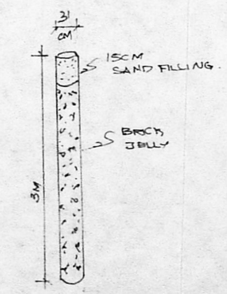
RAIN WATER PERCUSSION PIT (NTS)
